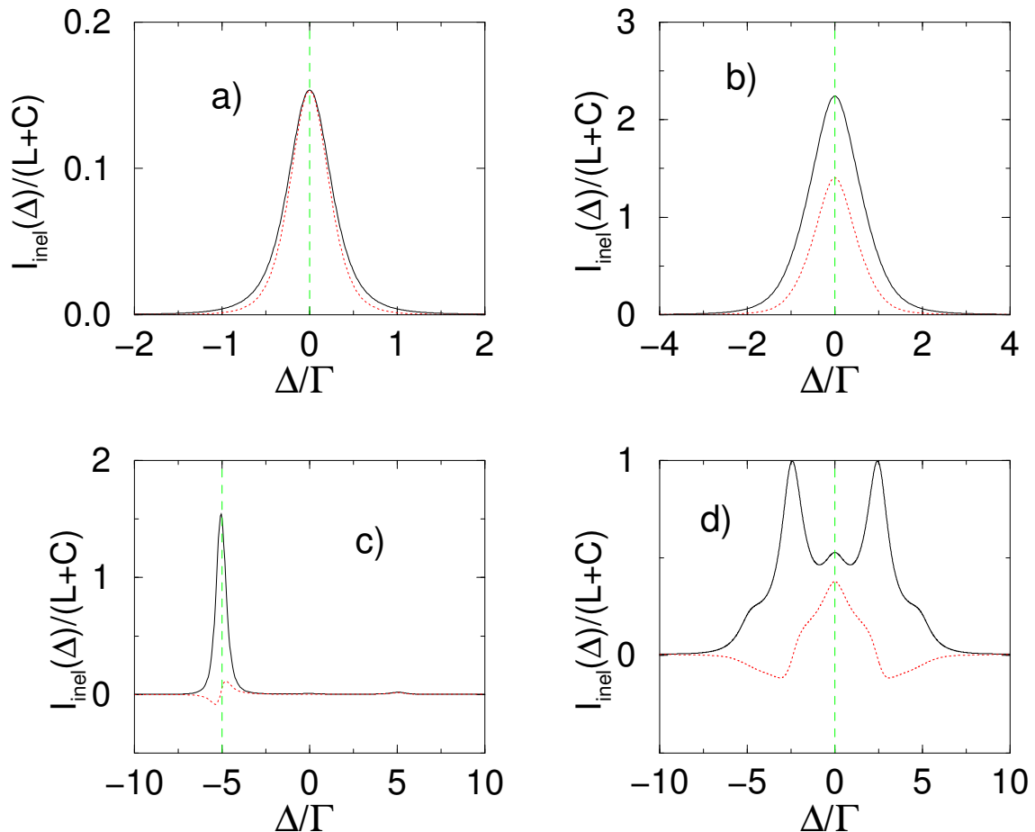
Figure 1: Backscattered light spectrum in the helicity-preserving polarization channel h \parallel h . The solid lines represent the ladder term (average background intensity value) and the dotted lines represent the crossed (interference) term. For both terms, the plotted values corresponds to I_{\text{inel}}(\Delta)/(C^{\text{tot}} + L^{\text{tot}}) , see Eq.(52), where C^{\text{tot}} + L^{\text{tot}} is the total (elastic plus inelastic) intensity scattered in the backward direction. The vertical dashed lines indicate the atomic transition frequency. \Delta corresponds to the scattered light angular frequency change with respect to the initial laser angular frequency ( \Delta = 0 means thus that light is radiated at \omega_L ). Graph (a) corresponds to an on-resonance saturation parameter s_0 = 0.02 and a laser detuning \delta = 0 ; Graph (b) to ( s_0 = 2, \delta = 0 ); Graph (c) to ( s_0 = 2, \delta = 5\Gamma ) and Graph (d) to ( s_0 = 50, \delta = 0 ). At low s_0 , the inelastic contribution to the total intensity is small and the ladder intensity is almost equal to the crossed one. For a larger saturation parameter, firstly the inelastic contribution becomes comparable to the elastic one and secondly, the crossed term becomes smaller than the ladder one. For a nonzero detuning, see graph (c), one clearly observes an asymmetry in the inelastic spectrum, which reflects the fact that the scattering cross-section of the atomic transition is maximal for resonant light: the symmetric inelastic spectrum emitted by a single atom is filtered out when scattered by the other one. At very large saturation (d), the structure of the radiated spectrum becomes rather complicated.
