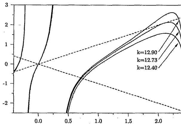
FIG. 3. Graph of the fixed-point equation (5) for k = k_c = 12.73 , k > k_c , k < k_c ; in the latter case (5) still allows for complex ghost solutions.
