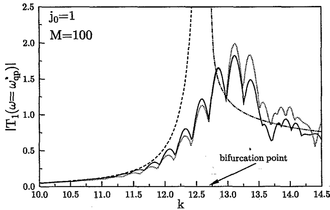
FIG. 4. Height of the quantum peak versus k near k_c . Full curve: exact quantum mechanics; dotted: semiclassics of Airy type, Eq. (10); dashed: ghost approximation ( k < k_c ); dash-dotted: standard Gutzwiller approximation ( k > k_c ).
