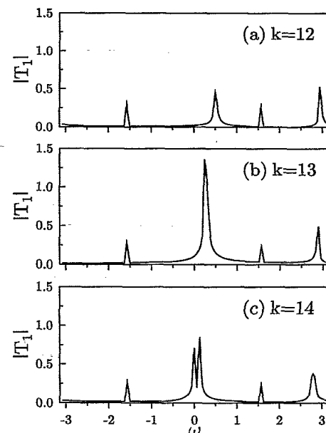
FIG. 1. Fourier transformed trace T_1(\omega; j_0 = 1, M = 100) of the Floquet operator of the kicked top for various values of the control parameter k : (a) below k_c = 12.73 with a ghost peak at \omega = 0.51 and three peaks corresponding to real periodic orbits; (b) slightly above k_c where the highest peak corresponds to an unresolved doublet due to two real periodic orbits; and (c) sufficiently far above k_c where the doublet is resolved.
